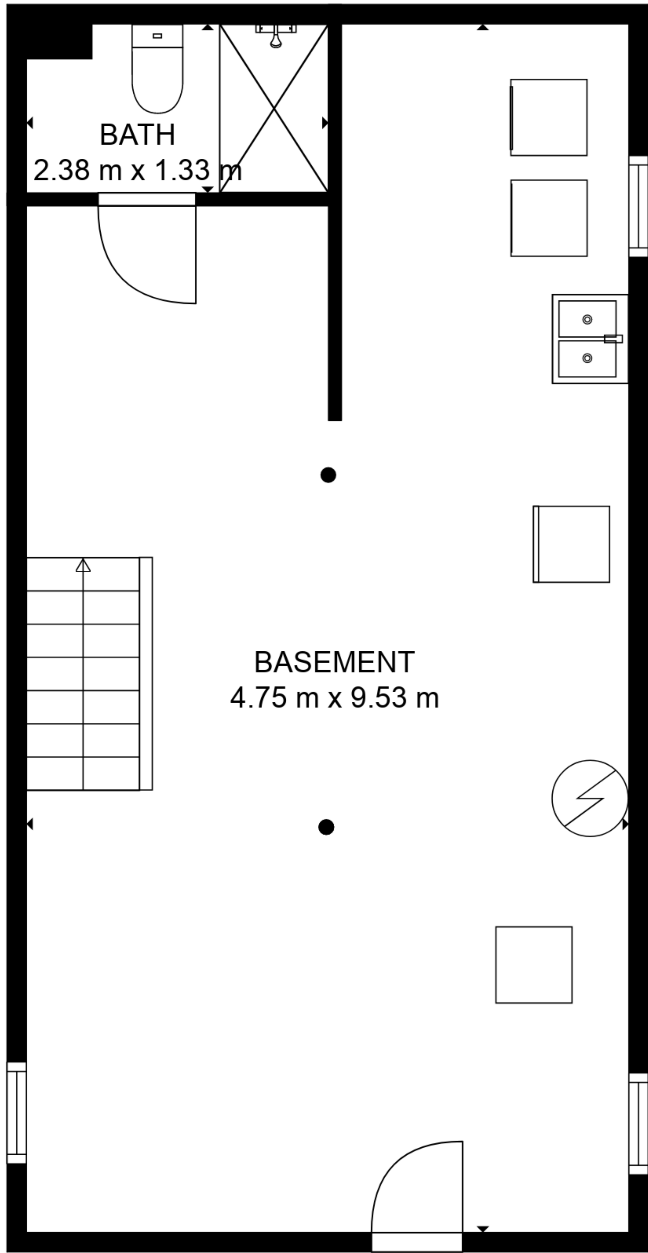
FLOOR 1
