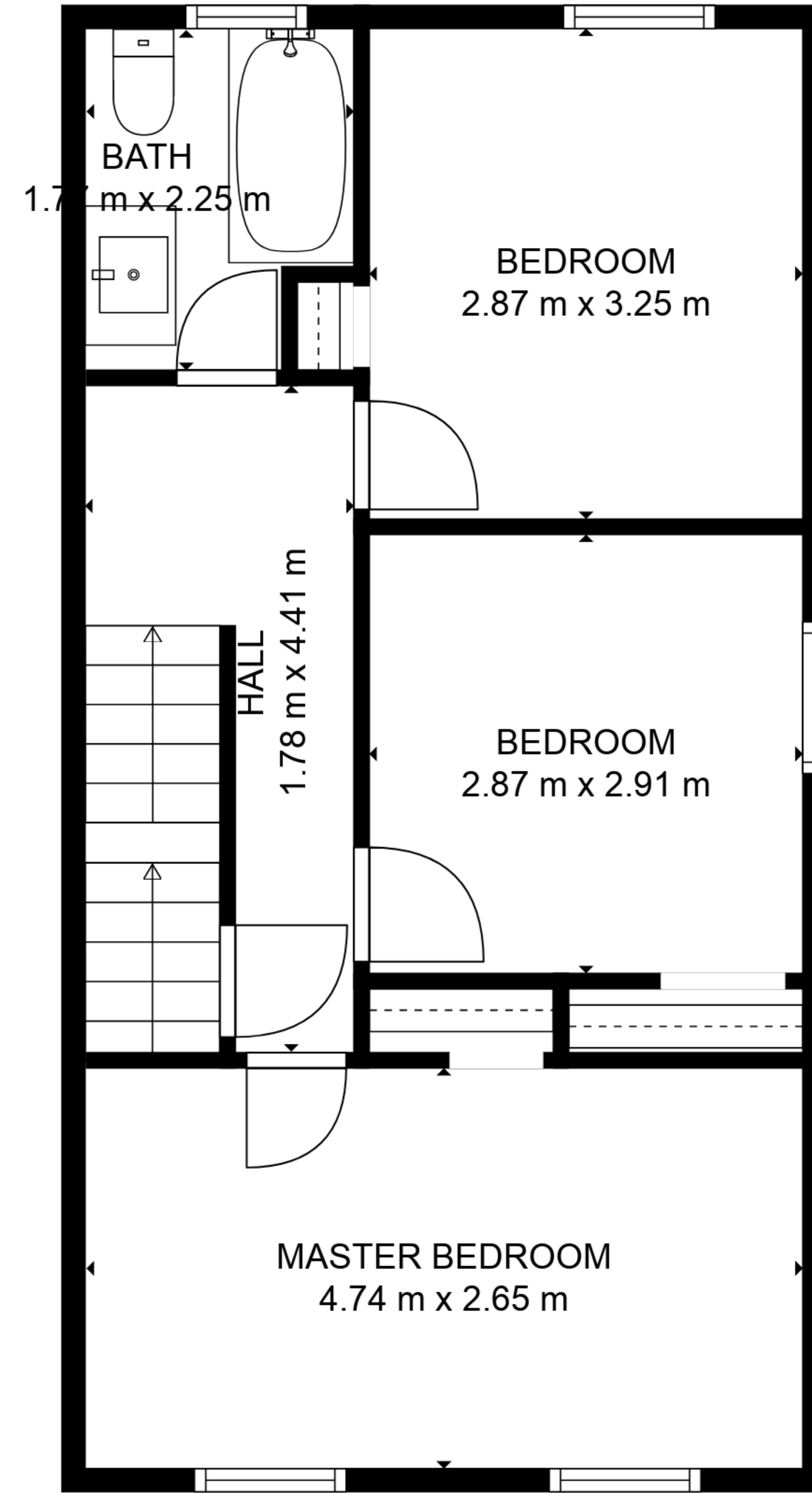
FLOOR 3
